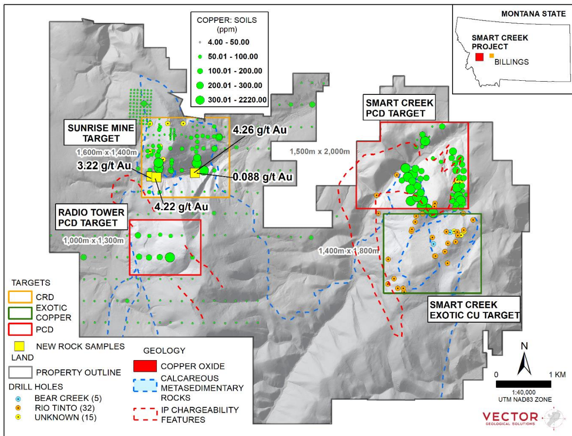
Figure 1. The Smart Creek Project, located in western Montana and the distribution of gold grades for newly received rock samples at the Sunrise Target. These new data demonstrate that robust gold grades exist up to 850 meters from the Sunrise Mine in porphyritic intrusions. The data indicates that there is a linkage between historically mined CRD mineralization and epithermal-porphyry transitional mineralization.
