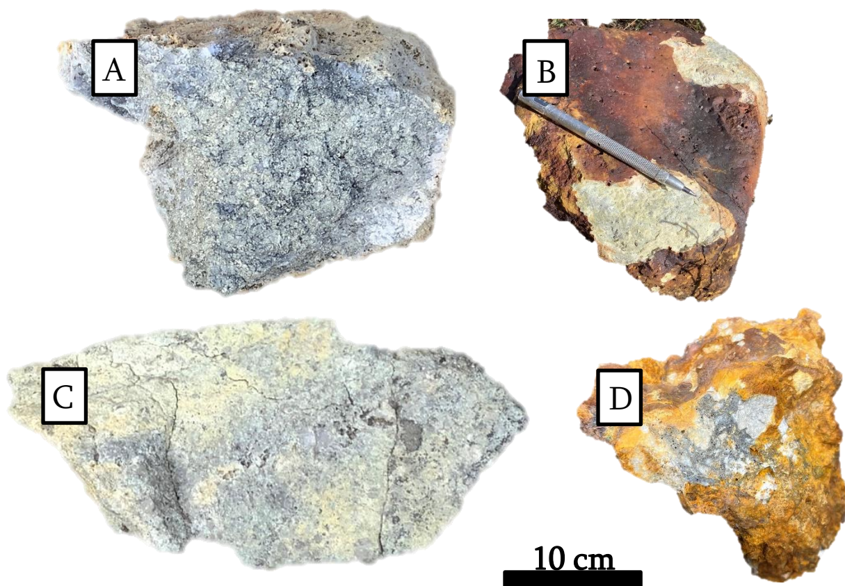
Figure 2. Rock sample photographs from the Sunrise Mine target area. New data demonstrate that robust gold grades exist up to 850 meters from the historic Sunrise Mine in porphyritic intrusions providing a linkage between historically mined CRD mineralization and epithermal-porphyry transitional mineralization. A) Sample 191902 (0.09 g/t Au); B) sample 191903 (4.26 g/t Au); C) sample 191904 (3.22 g/t Au); sample 191905 (4.22 g/t Au).
